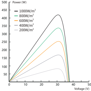
Power-Voltage Curve(420W)
